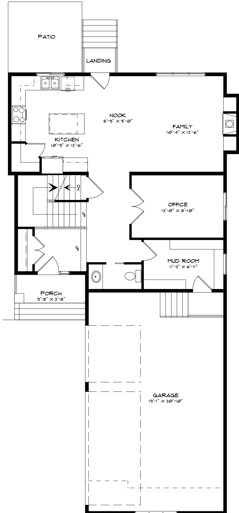
MAIN FLOOR PLAN 918 SQ.FT.
