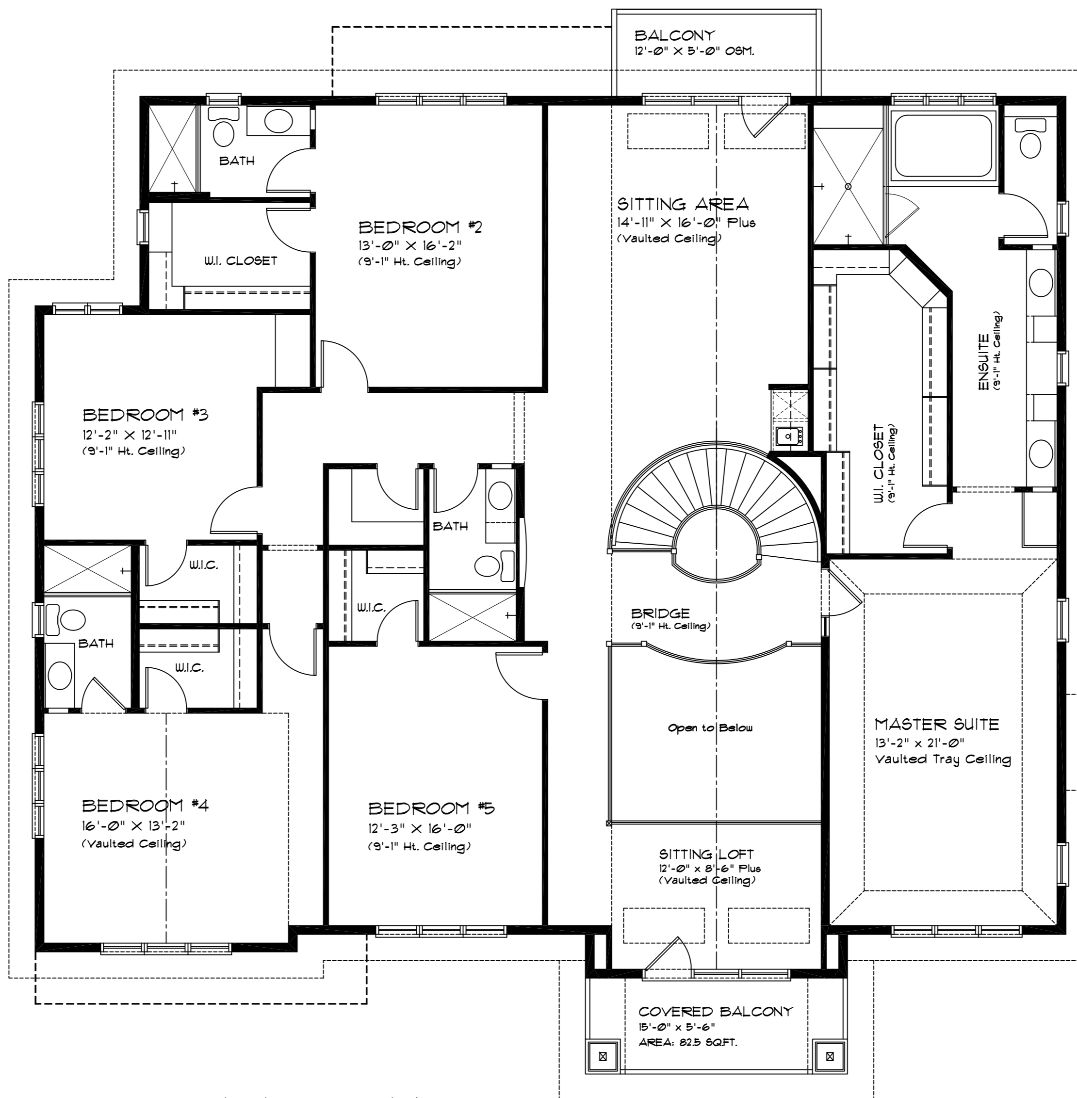
Proposed Upper Floor AREA: 2628 SQ.FT.
